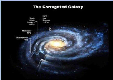
Astrophysics
