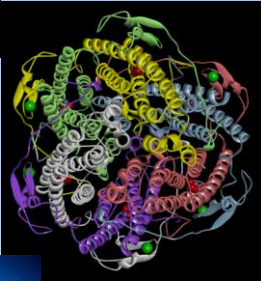
Biophysics
