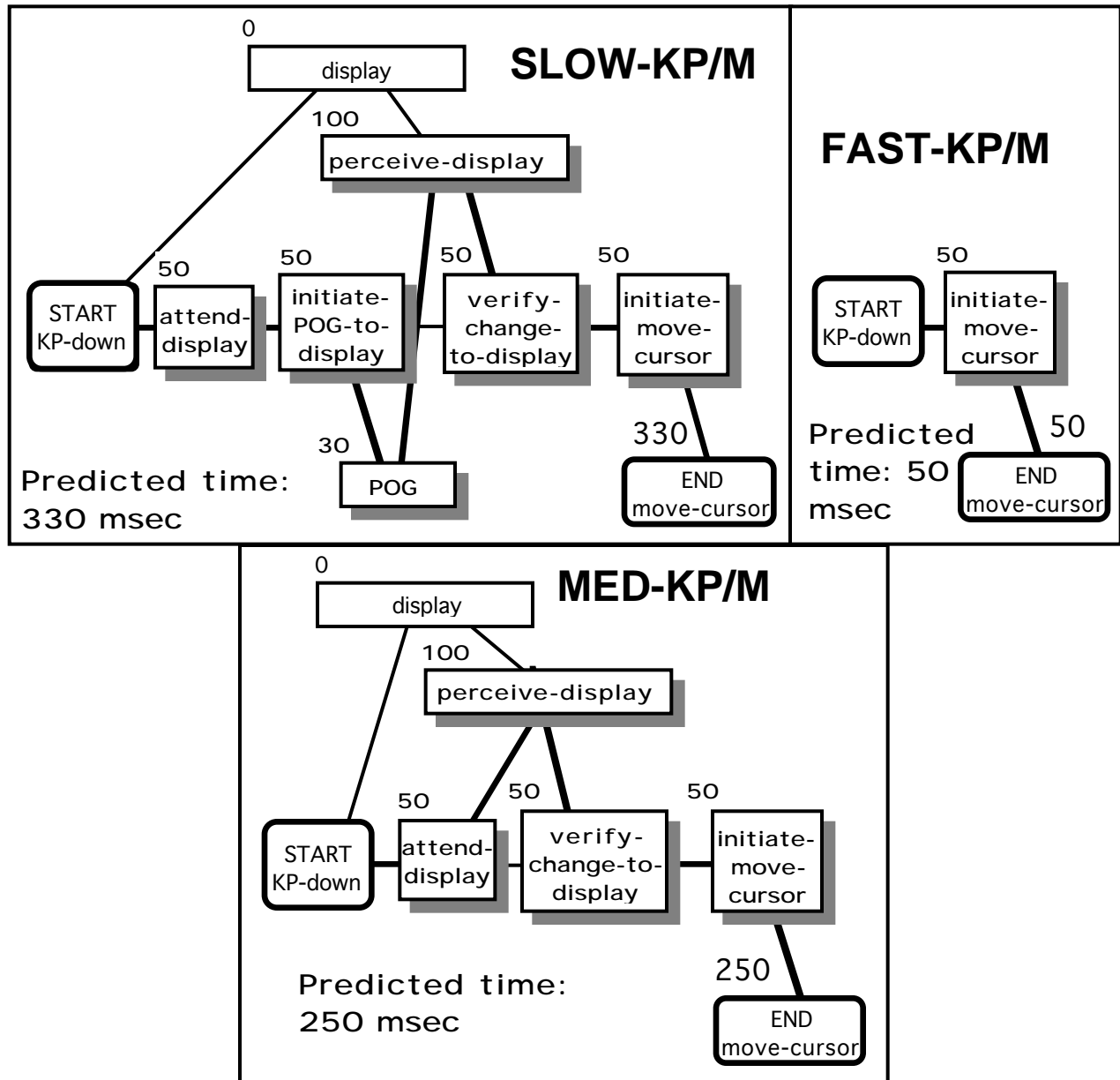
Figure 1: Microstrategies for KEYPRESS-MOVE. The critical path is indicated by bold lines connecting shadowed boxes.
