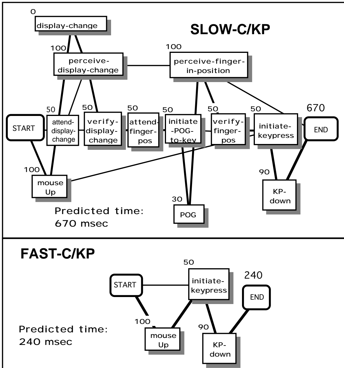
Figure 2: Microstrategy for CLICK-KEYPRESS. Top: SLOW-C/KP. Bottom: FAST-C/KP. The critical path is indicated by bold lines connecting shadowed boxes.
