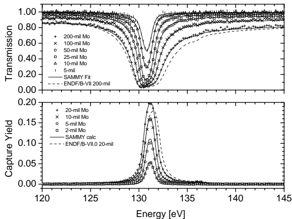
Fig. 1. Measured Molybdenum transmission (top) and capture data plotted with the SAMMY fit. A calculation with the ENDF/B-VII.0 resonance parameters is also shown (1 mil = 0.00254 cm).
