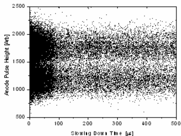
Fig. 5. – A plot of the anode pulse height which is proportional to the fission fragment energy vs. the neutron slowing down time.
