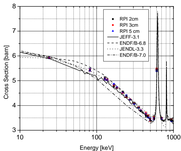
Fig 4 – Total cross section of Beryllium measured using an iron filtered beam
