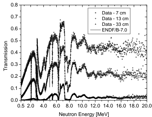
Fig. 3. Measured graphite (carbon) transmission for three sample thicknesses.
