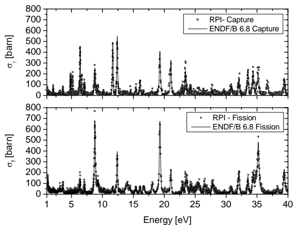
Fig. 2. Results of a simultaneous measurement of the fission and capture cross section of ^{235}\text{U} using the RPI multiplicity detector.
